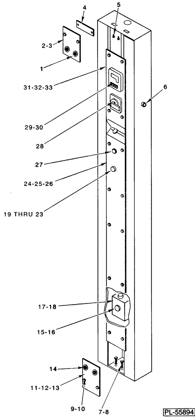
HUMIDIFIER CONTROL PANEL
